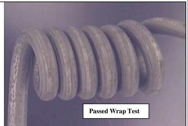
Figure XII: Bezinal: Heat Treated at 315 0 C for a soak time of 14 Hours
