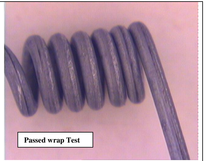
Figure XVI: Beznal: Heat Treated at 350 0 C for a soak time of 16 weeks.
