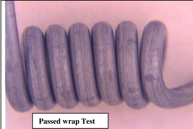
Figure XIII: Beznal: Heat Treated at 315 0 C for a soak time of 4 weeks.
