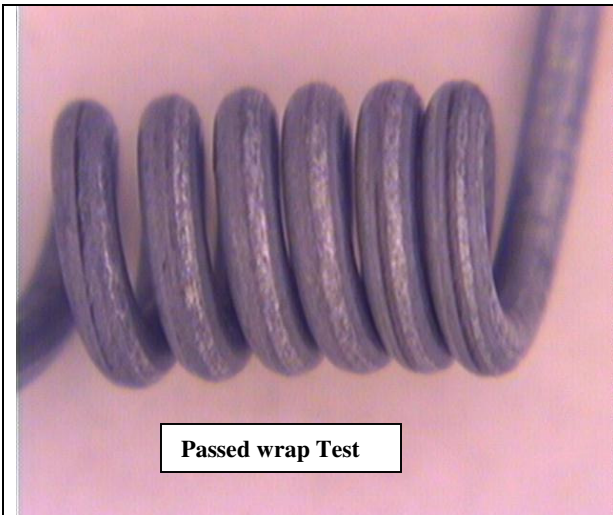
Figure XV: Beznal: Heat Treated at 350 0 C for a soak time of four weeks.
