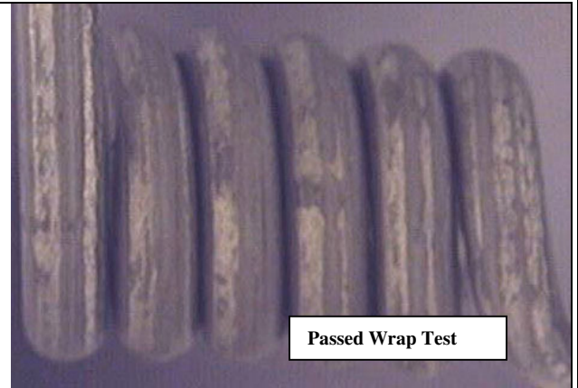
Figure X: Bezinal: Heat Treated at 250 0 C for a soak time of 1 week
