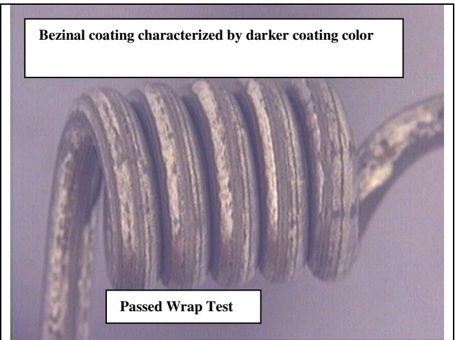
Figure II: Bezinal: Pre Heat Treated
