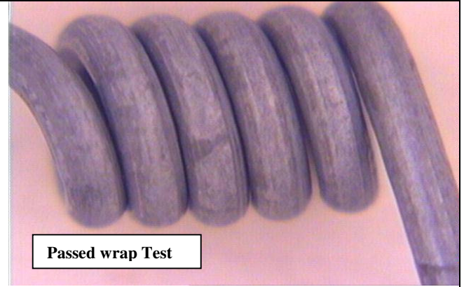
Figure XIV: Beznal: Heat Treated at 315 0 C for a soak time of 16 weeks.
