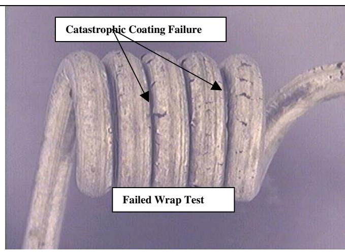
Figure VIII: Galvanized: Heat Treated at 250 0 C for a soak time of 72 Hours (Three days)
