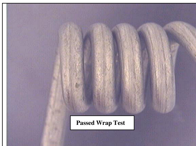
Figure VII: Galvanized: Heat Treated at 250 0 C for a soak time of 48 Hours (Two days)
